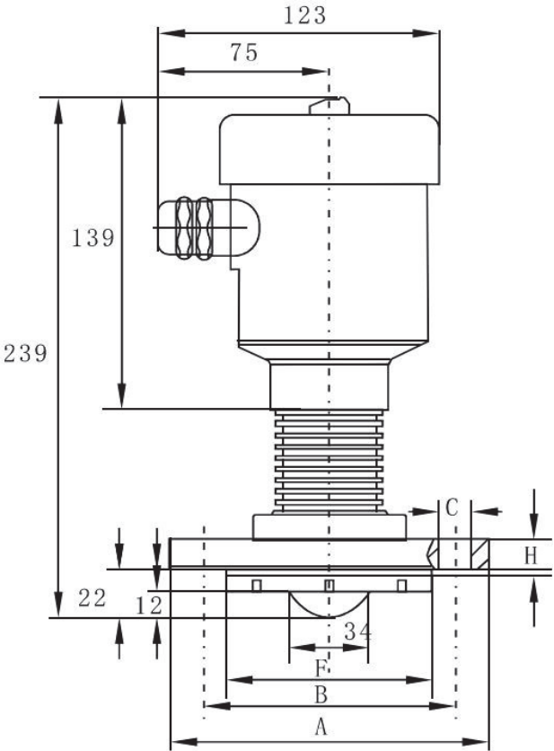
Fig.6 Flange with encapsulated antenna system (High temperature&press)
