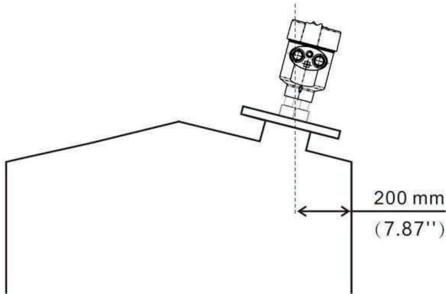
Fig. 9 Example for avoiding false echo
