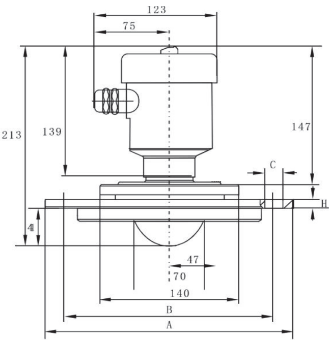
Fig.3 Universal Type (Normal temperature type)
