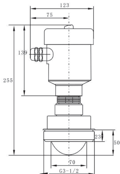
Fig.2 Thread connection (High temperature type)
