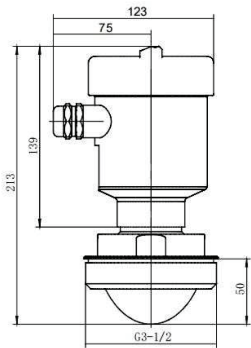
G3 1/2 Thread
